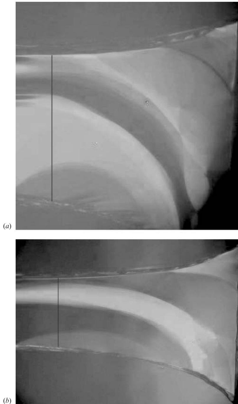
Figure 6. (a) Strip of an Inter3/05 film between two parallel edges with initial distance \ell_0 = 2.5 mm in the relaxed state, observed in blue light ( \lambda = 488 nm). The initial film thickness is between 170 and 400 nm. (b) The same film after uniaxial expansion by 67%. The image sizes are (a) 1.26 \times 1.25 mm (a) and (b) 1.62 \times 1.49 mm.
